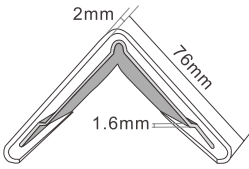
HS-607B Side width:76x76mm Side length:3m/pc Corner angle: 90°
