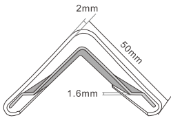
HS-605B Side width:50x50mm Side length:3m/pc Corner angle: 90°
